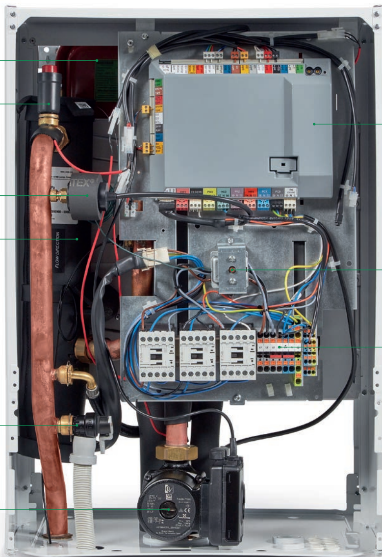
Circulating pump
