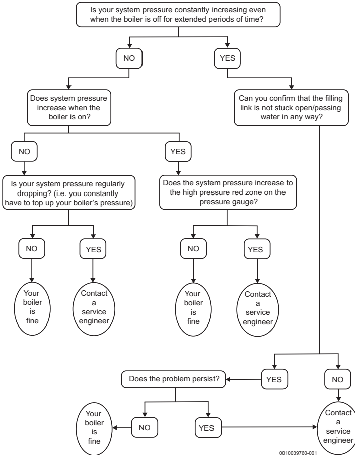
Fig. 9 System gassing trouble-shooting flow chart
